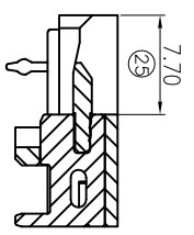
SECTION F-F SCALE 1:1
